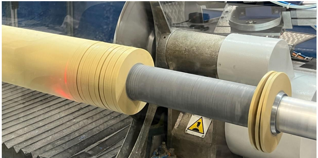
Cutter assembly with spacers and cutters
