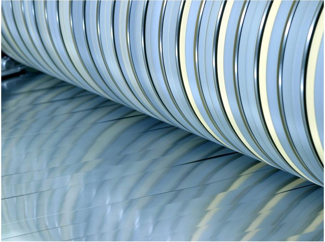
Cutter assembly with spacers and cutters
